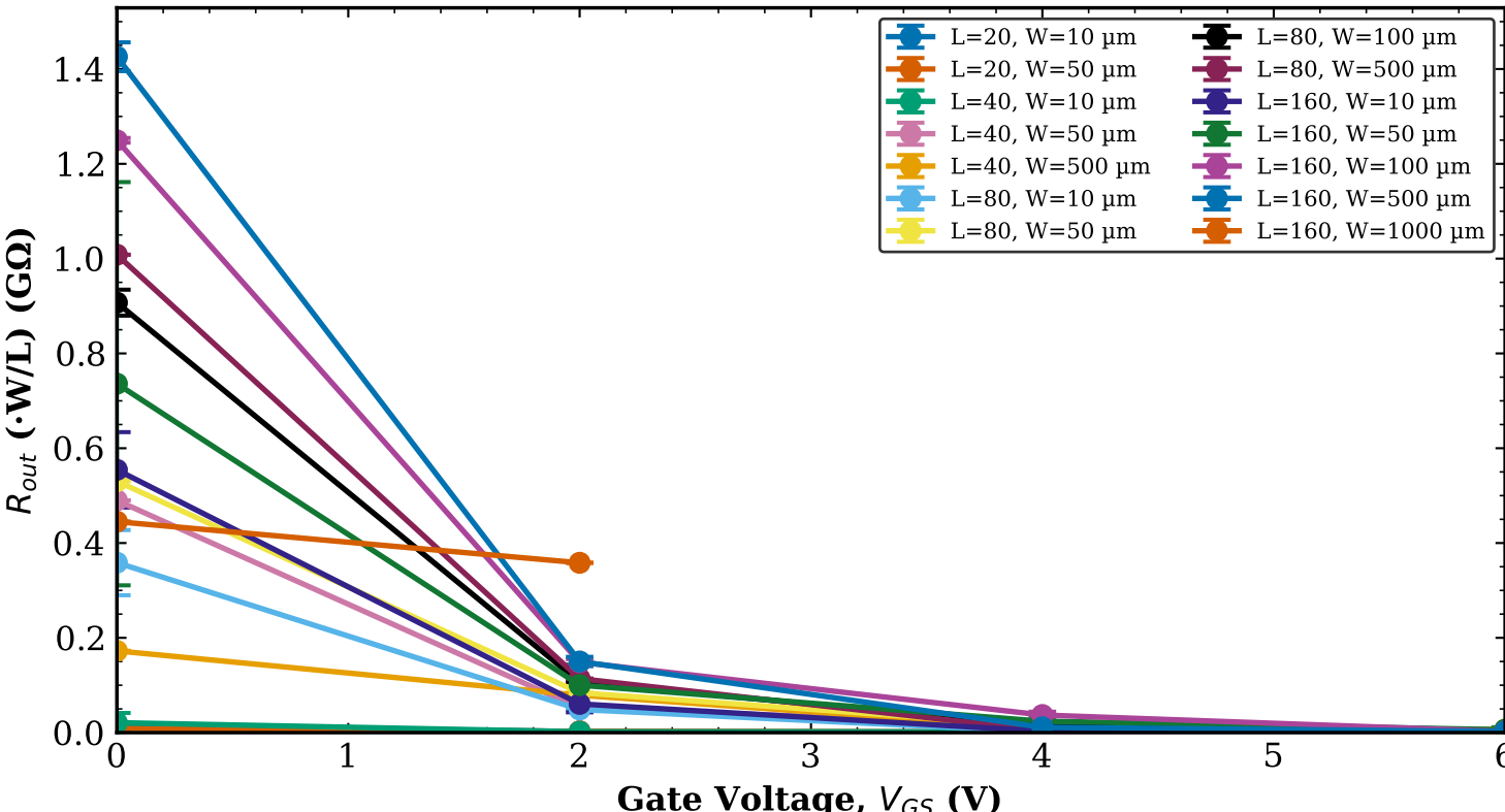
TFT2 Combined (Tr. 1 & 2) Output Resistance vs V_{GS}
